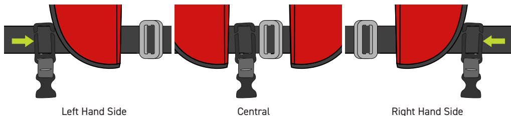
Fig 2.2A - Depending on the make and model, the crotch strap may be fitted to the left, right or centre of the life jacket. Ensure there is sufficient space at each potential attachment point and discount any position that may cause interference or obstruct adjustment of the waist belt.
